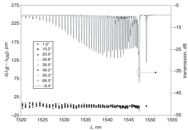
Fig. 2 Transmission spectrum of weakly tilted FBG and differential wavelength shift due to temperature changes
