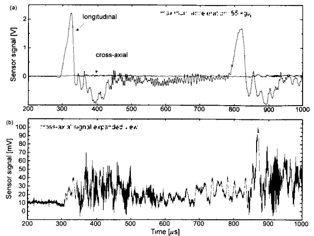
Fig. 7. Cross-axis sensitivity measurement of the fiber Bragg sensor. The curves labeled cross-axis and longitudinal in Fig. 7(a) show respectively the sensor response when a 85 kg_n acceleration is applied perpendicular (cross-axis) to the axis of the sensor fiber and same acceleration is applied along (longitudinal) the sensor fiber axis. Figure 7(b) is the same signal redrawn with a higher amplitude sensitivity.
