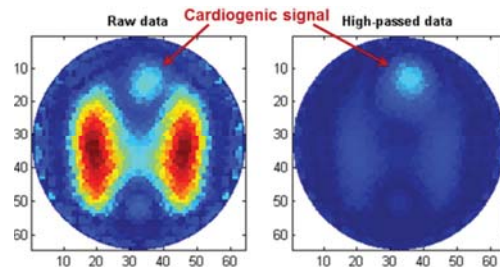
Figure 3: AC Energy of each pixel in the reconstructed image sequence without (left) and with (right) the high-pass filter.
