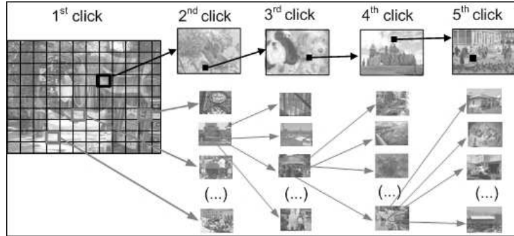
Fig. 1. CCP passwords can be regarded as a choice-dependent path of images
