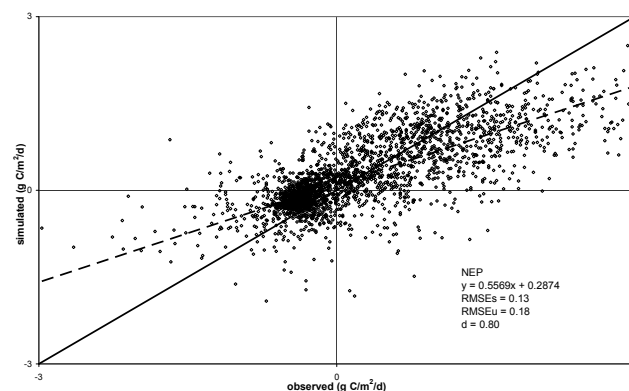
Fig. 5. The scatter plot of observed and simulated daily NEP for 1999–2006. The solid black line indicates the 1:1 line and the dashed line is the best fit relationship between the observations and the simulated NEP.
